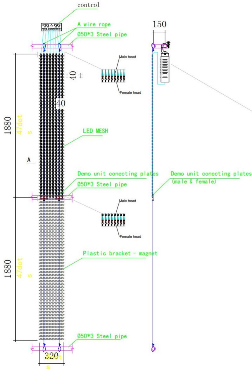
LED module splicing diagram
